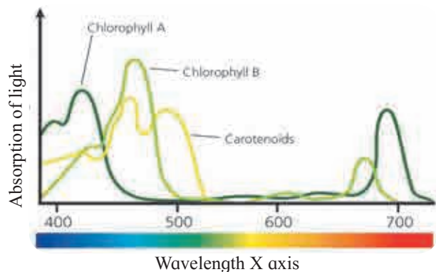
Graph 12.3 Absorption spectrum
