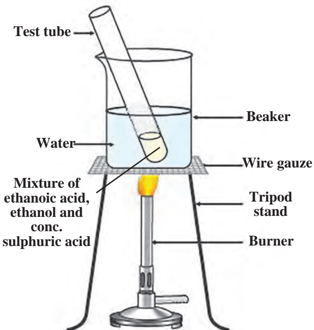
9.25 Esterification Reaction
